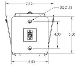
Wall Mount Side
